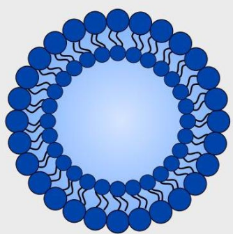
Liposome 50 - 450 nm
