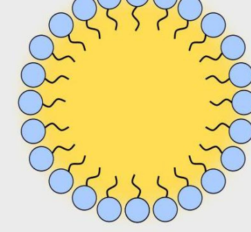
Nanoemulsion 10 - 1000 nm
