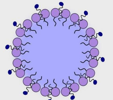
Polymer nanoparticle
