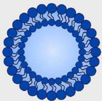
Liposome 50 - 450 nm
