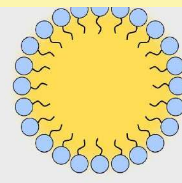
Nanoemulsion 10 - 1000 nm
