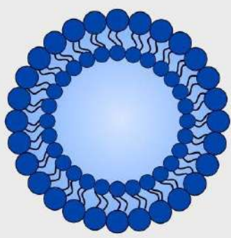
Liposome 50 - 450 nm
