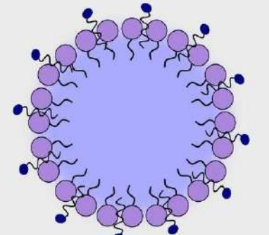
Polymer nanoparticle
