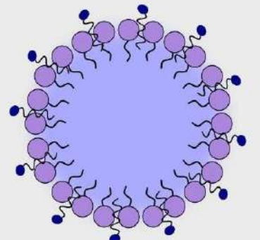
Polymer nanoparticle
