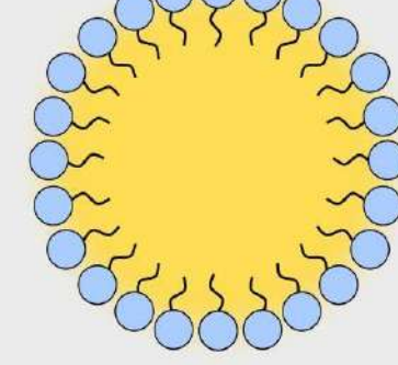
Nanoemulsion 10 - 1000 nm
